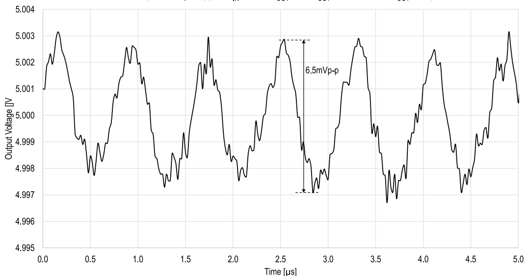
171930601 Output Voltage Ripple, V_{\text{IN}} = 24\text{V} , V_{\text{OUT}} = 5\text{V} , I_{\text{OUT}} = 300\text{mA} and C_{\text{OUT}} = 68\mu\text{F}
