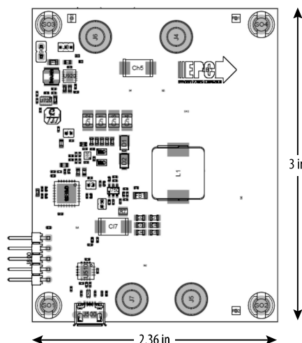
Figure 12: EPC9162 mechanical dimensions
