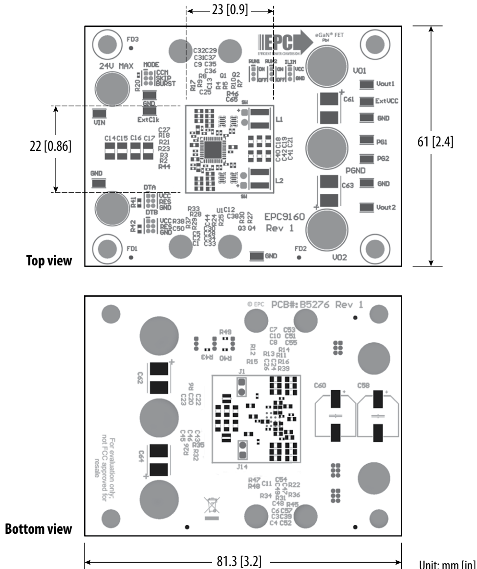
Figure 9: Mechanical dimensions
