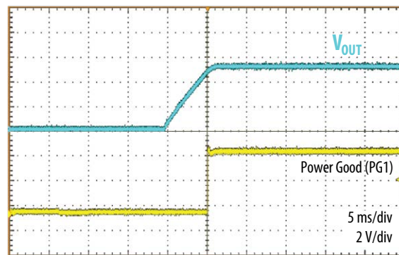
Figure 4: Startup waveform: V_{IN} = 24 V, V_{OUT1} = 5 V ( I_{lim} = VCC )
