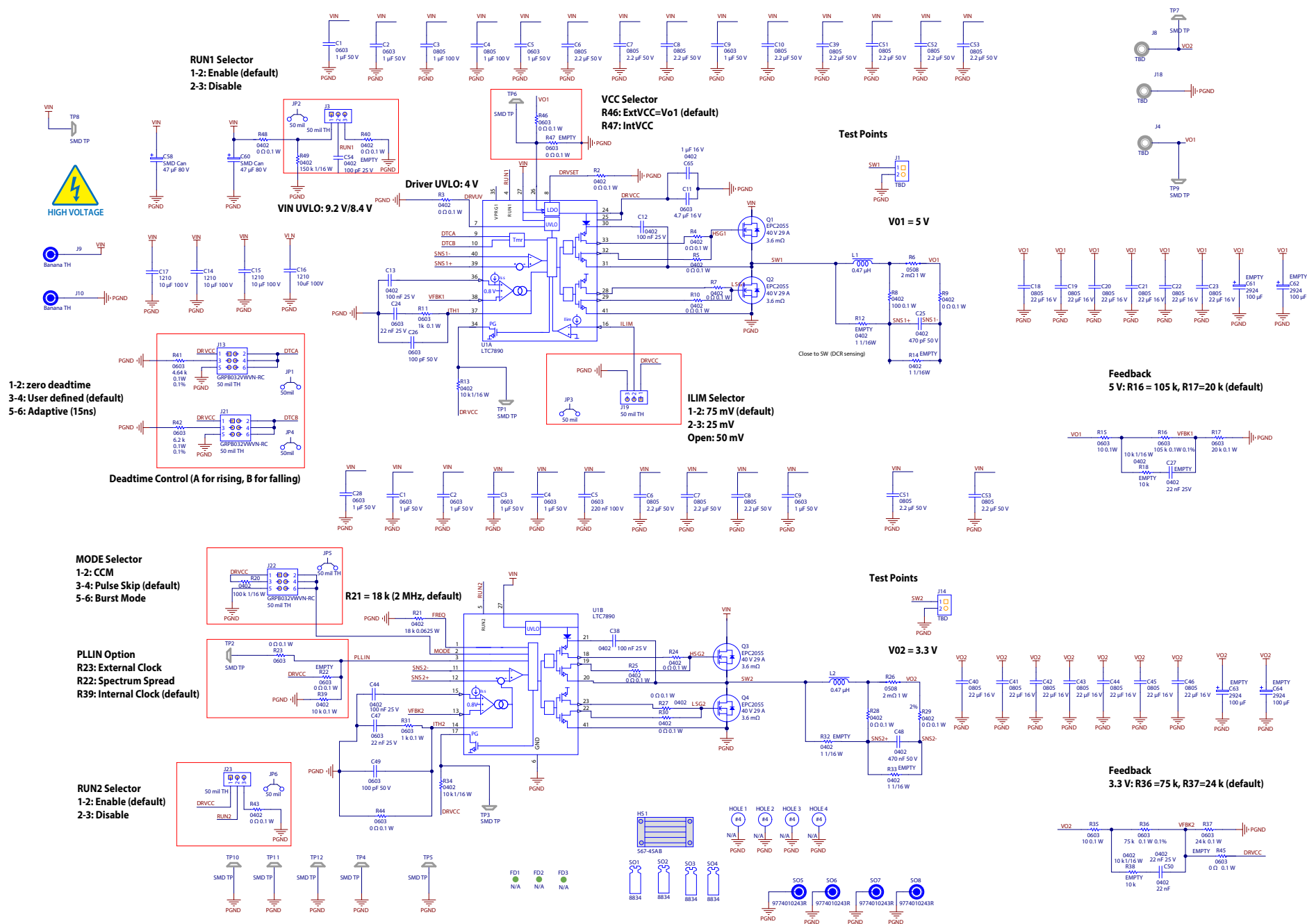
Figure 10: EPC9160 schematic
