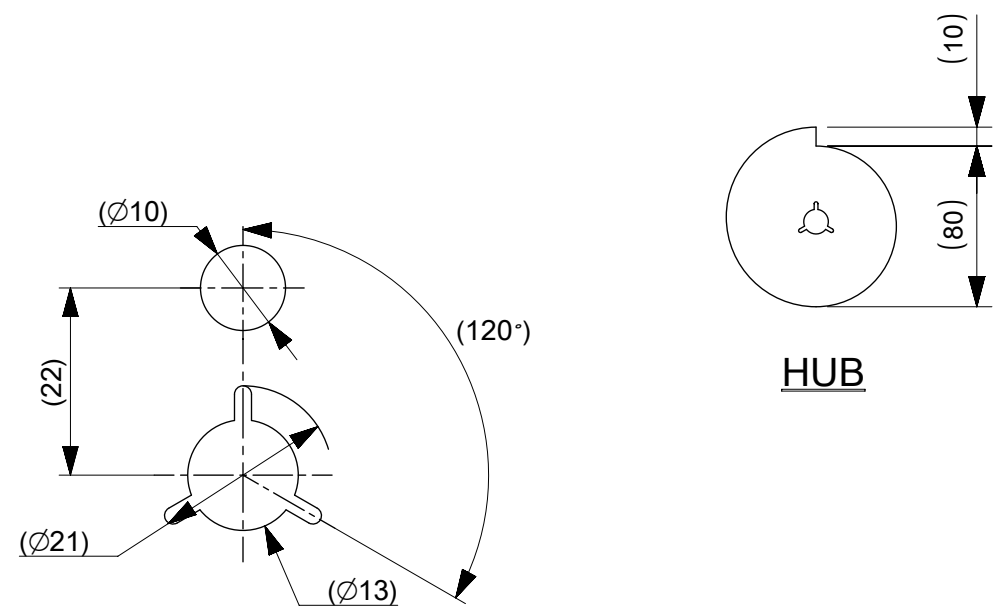
DETAIL "F"
