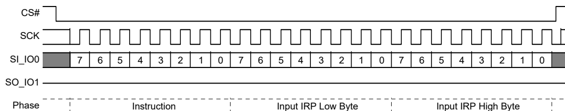
Figure 109. IRP Program (IRPP) Command
