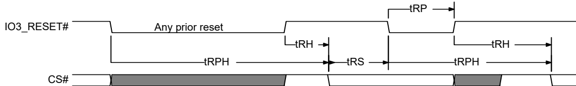
Figure 141. Hardware Reset when Quad or QPI Mode and IO3 / RESET# are Enabled
