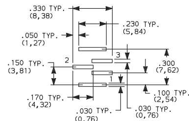
SV1 Terminal Style GS01 Models
