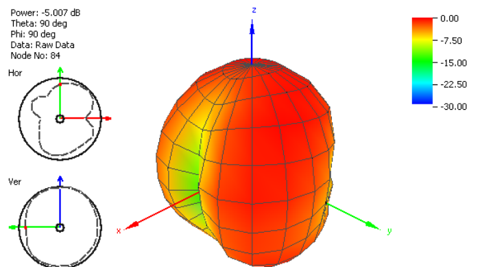
Figure 19. Radiation Pattern at 925 MHz of FXUB70 Port 2.
