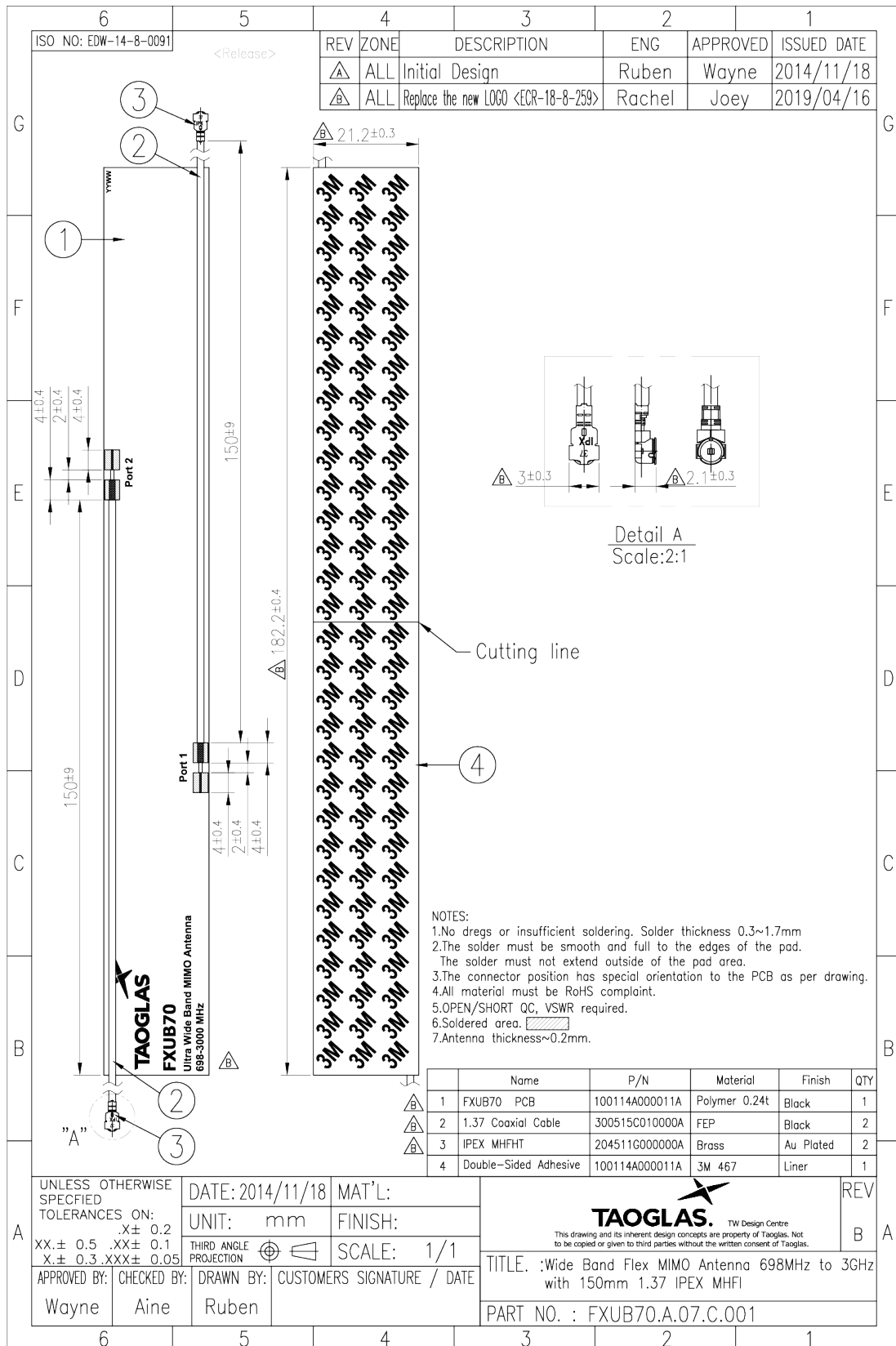
Figure 34. Mechanical drawing of FXUB70 Antenna.
