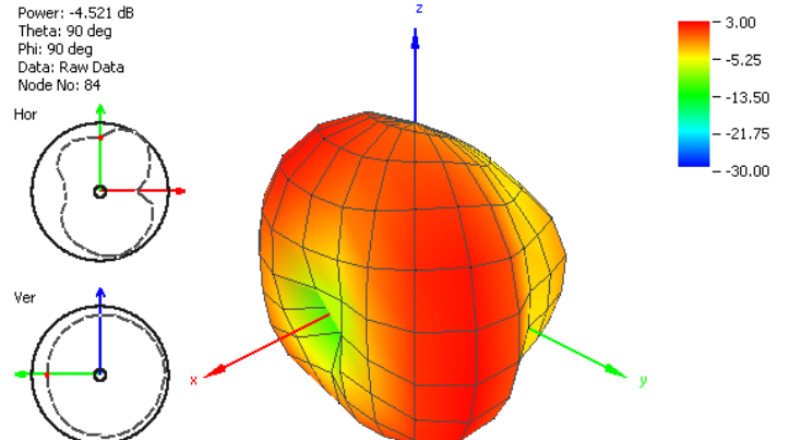
Figure 27. Radiation Pattern at 1950 MHz of FXUB70 Port 2.
