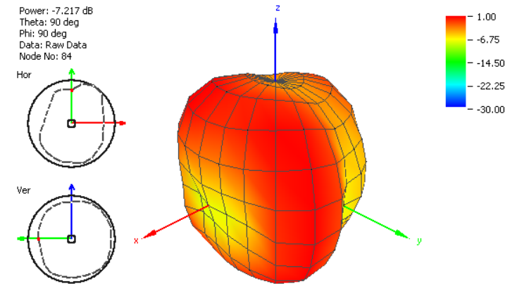
Figure 23. Radiation Pattern at 1750 MHz of FXUB70 Port 2.
