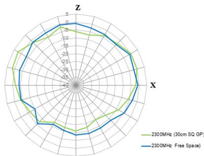
XZ Plane
