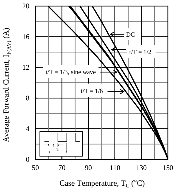
Figure 1. I_{F(AV)} vs. T_C ( T_J = 150\text{ }^{\circ}\text{C} , V_R = 0\text{ V} )
