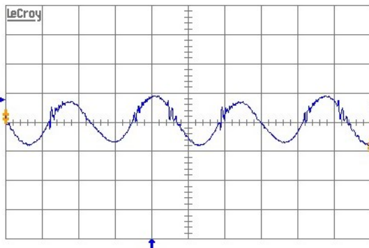
Figure 10. Output voltage ripple (20 mV/div.) at full rated load current into a resistive load with C_o = 10\text{ }\mu\text{F} tantalum + 1 \mu\text{F} ceramic and V_{in} = 48\text{ V} . Time scale: 1 \mu\text{s} /div.
