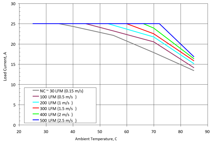
Figure 1. Available load current vs. ambient air temperature and airflow rates for SSQE48T25025 converter mounted vertically with air flowing from pin 1 to pin 3, V_{in} = 48 V . Note: NC – Natural convection
