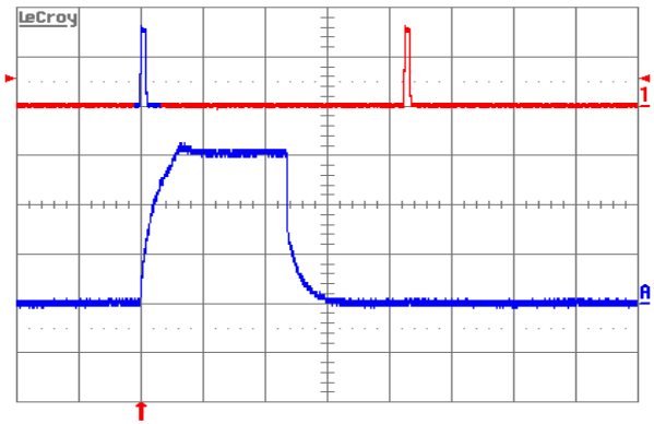
Figure 15. Load current (top trace, 20 A/div., 50 ms/div.) into a 10 mΩ short circuit during restart, at Vin = 48 V. Bottom trace (10 A/div., 2 ms/div.) is an expansion of the on-time portion of the top trace.
