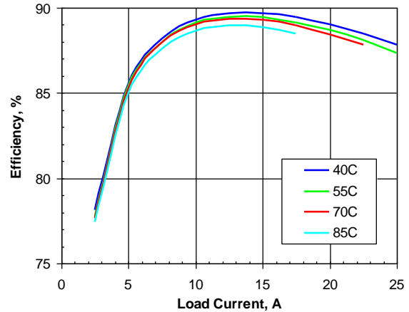
Figure 3. Efficiency vs. load current and ambient temperature for SSQE48T25025 converter mounted vertically with V_{in}=48\text{V} and air flowing from pin 1 to pin 3 at a rate of 200LFM (1.0m/s).
