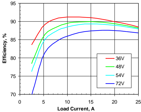
Figure 2. Efficiency vs. load current and input voltage for SSQE48T25025 converter mounted vertically with air flowing from pin 1 to pin 3 at a rate of 300 LFM (1.5 m/s) and T_a=25^{\circ}\text{C} .
