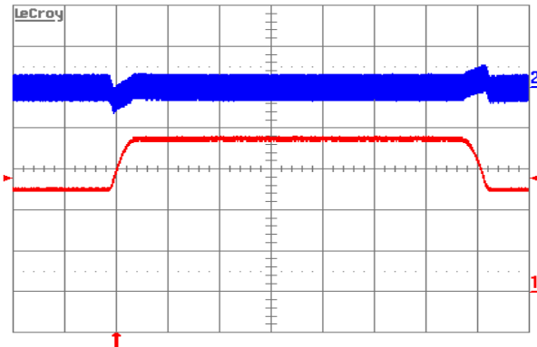
Figure 8. Output voltage response to load current step-change (12.5A–18.75A–12.5A) at V_{in}=48V . Top trace: output voltage (100mV/div.). Bottom trace: load current (5A/div.). Current slew rate: 0.1A/\mu s . C_o=1\mu F cer+ 10\mu F tant. Time scale: 0.2ms/div
