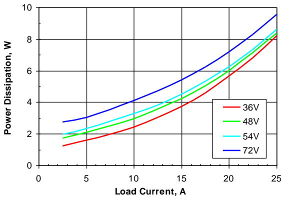
Figure 4. Power dissipation vs. load current and input voltage for SSQE48T25025 converter mounted vertically with air flowing from pin 1 to pin 3 at a rate of 300 LFM (1.5 m/s) and T_a = 25^{\circ}\text{C} .
