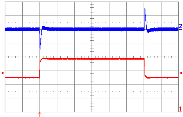
Figure 9. Output voltage response to load current step-change (12.5A–18.75A–12.5A) at V_{in}=48V . Top trace: output voltage (100 mV/div.). Bottom trace: load current (5A/div.). Current slew rate: 5A/\mu s . C_o=470\mu F POS+ 1\mu F cer. Time scale: 0.2ms/div.
