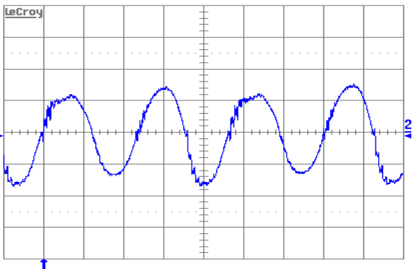
Figure 10. Output voltage ripple (20 mV/div.) at full rated load current into a resistive load with C_o = 10 \mu F tantalum + 1 \mu F ceramic and V_{in} = 48 V . Time scale: 1 \mu s /div.
