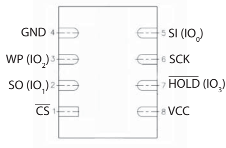
Figure 1-6. 8-pad USON (Bottom View)
