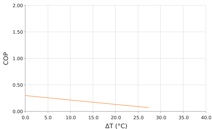
Coefficient of Performance (COP = Q_c/P_{in} ) T_{hot} = 85\text{ }^{\circ}\text{C} | Current = 4.2 Amps
