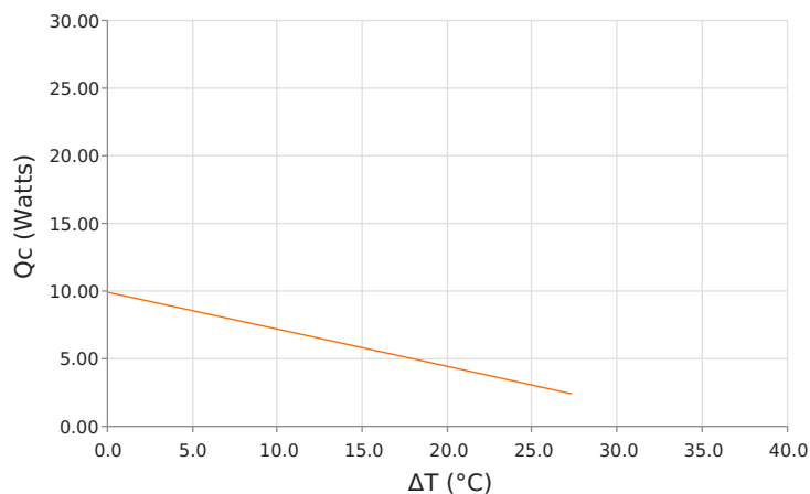
Heat Pumped at Cold Side ( Q_c ) T_{hot} = 85\text{ }^{\circ}\text{C} | Current = 4.2 Amps
