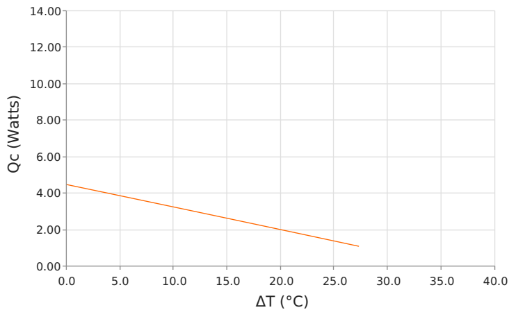
Heat Pumped at Cold Side ( Q_c ) T_{hot} = 85\text{ }^{\circ}\text{C} | Current = 2.5 Amps
