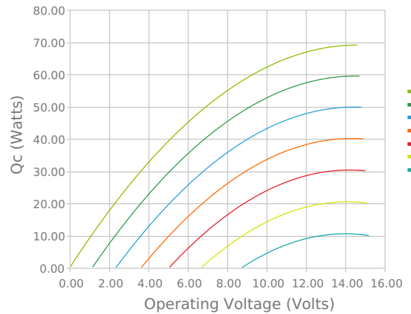
Heat Pumped at Cold Side T_{\text{hot}} = 27^\circ\text{C}
