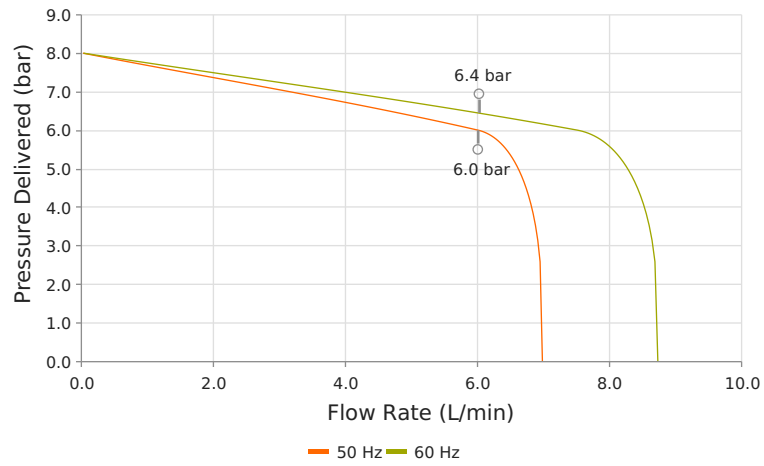
WL3004 - Pump Curve
