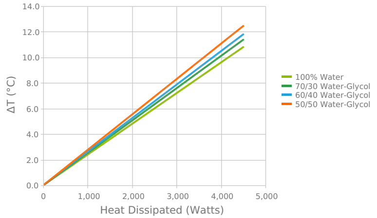
WL3004 Fluid Inlet/Outlet Temperature Difference ( \Delta T ) @ Nominal Flow 6 L/min
