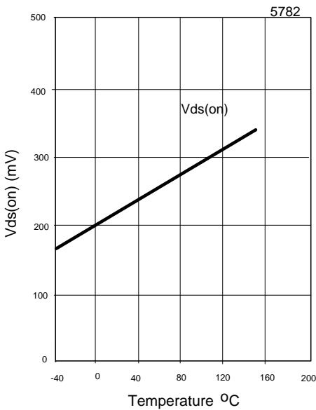
Typical Saturation Voltage vs. Temperature VDD=12V, I out =20mA
