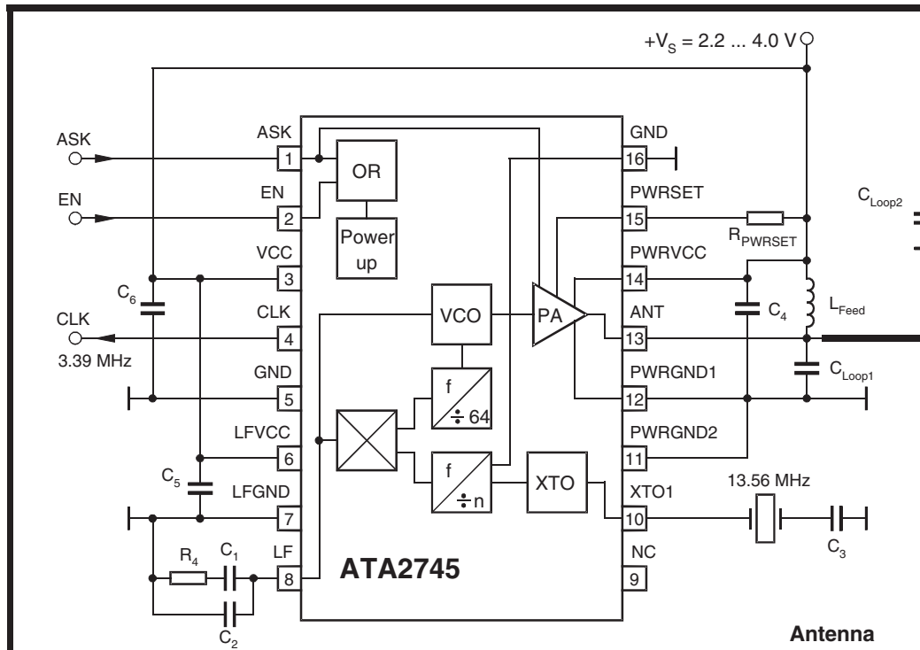
Figure 5-2. Application Circuit
