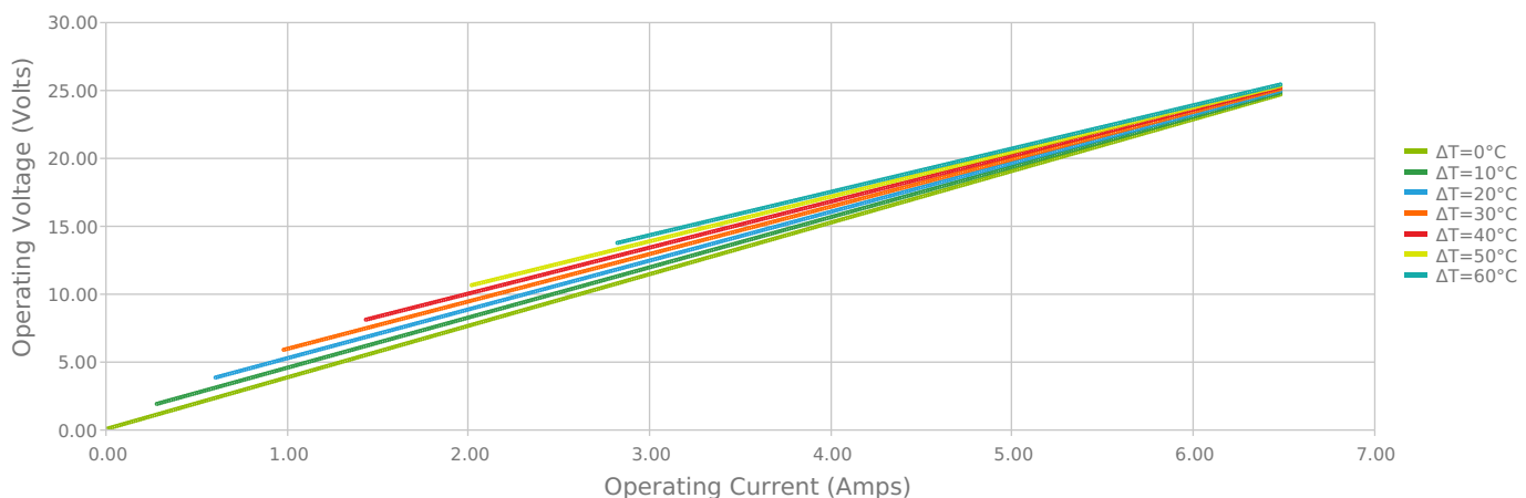
Current vs Voltage (I vs V) T_{hot} = 27^\circ\text{C}
