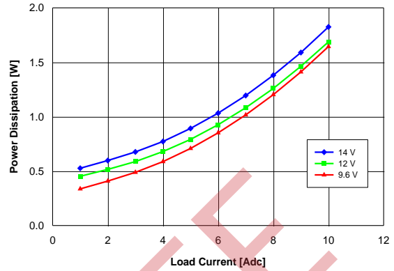
Fig. 1.5V.4: Power loss vs. load current and input voltage for YNL12S10015 converter mounted vertically with air flowing at a rate of 200 LFM (1 m/s) and T_a = 25^\circ\text{C} .
