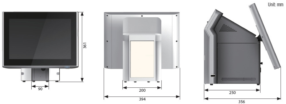
Figure 1.1 Dimensions of UPOS-3150
