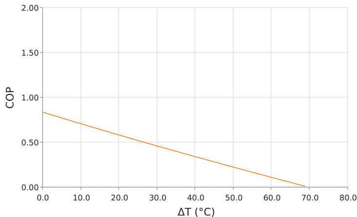
Coefficient of Performance (COP = Q_c/P_{in} ) T_{hot} = 27\text{ }^{\circ}\text{C} | Current = 1.8 Amps
