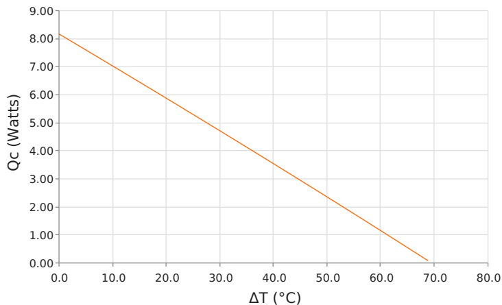
Heat Pumped at Cold Side ( Q_c ) T_{hot} = 27\text{ }^{\circ}\text{C} | Current = 1.8 Amps
