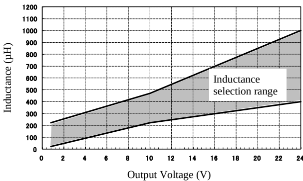
Figure 12-2. Inductance Selection Range in f = 350 \text{ kHz}
