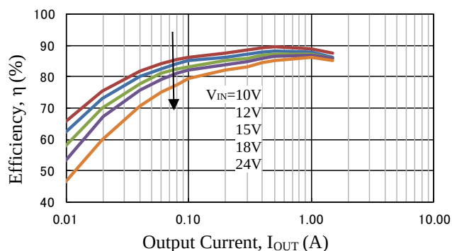
Figure 5-1. Efficiency ( V_{OUT} = 3.3 V)
