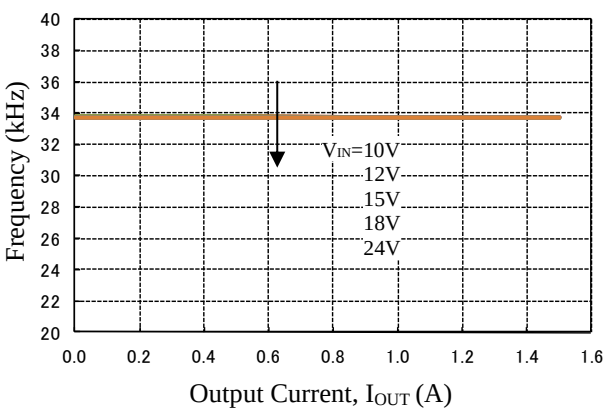
Figure 5-8. Operating Frequency
