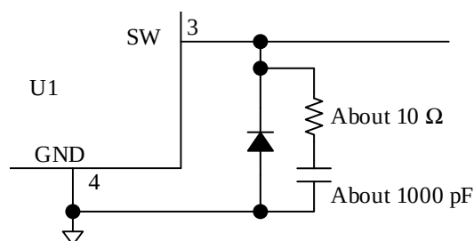
Figure 12-11. SW pin peripheral circuit
