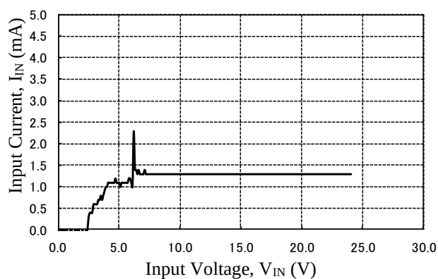
Figure 5-6. IN Pin Sink Current at No Load
