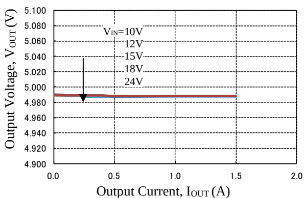
Figure 5-5. Load Regulation
