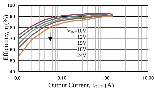
Figure 5-2. Efficiency ( V_{OUT} = 5.0 V)
