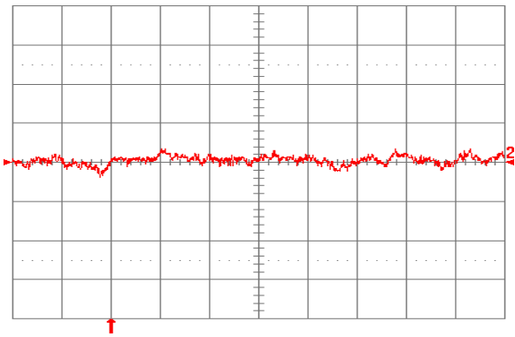
Fig. 12: Input reflected ripple current, i_s (10 mA/div), measured through 10\ \mu\text{H} at the source at full rated load current and V_{in} = 48\ \text{V} . Refer to Fig. 11 for test setup. Time scale: 1\ \mu\text{s}/\text{div} .
