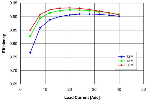
Fig. 3: Efficiency vs. load current and input voltage for converter mounted vertically with air flowing from pin 3 to pin 1 at a rate of 300 LFM (1.5 m/s) and T_a = 25^{\circ}\text{C} .
