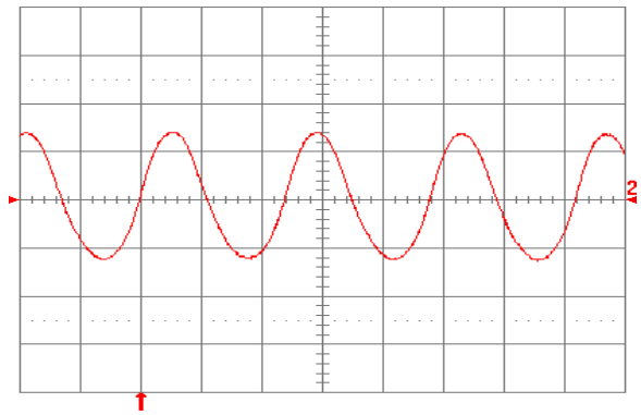
Fig. 13: Input reflected ripple current, i_c (100 mA/div), measured at input terminals at full rated load current and V_{in} = 48\ \text{V} . Refer to Fig. 11 for test setup. Time scale: 1\ \mu\text{s}/\text{div} .
