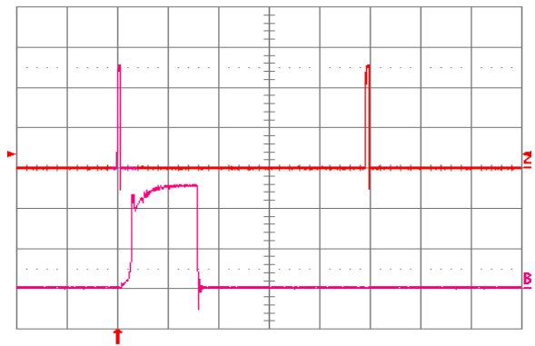
Fig. 15: Load current (top trace, 20\ \text{A}/\text{div} , 20\ \text{ms}/\text{div} ) into a 10\ \text{m}\Omega short circuit during restart, at V_{in} = 48\ \text{V} . Bottom trace ( 20\ \text{A}/\text{div} , 1\ \text{ms}/\text{div} ) is an expansion of the on-time portion of the top trace.
