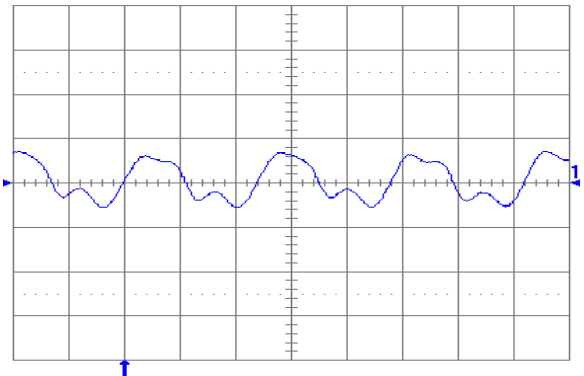
Fig. 10: Output voltage ripple (20 mV/div.) at full rated load current into a resistive load with C_o = 10\ \mu\text{F} tantalum + 1 \mu\text{F} ceramic and V_{in} = 48\text{ V} . Time scale: 1 \mu\text{s} /div.
