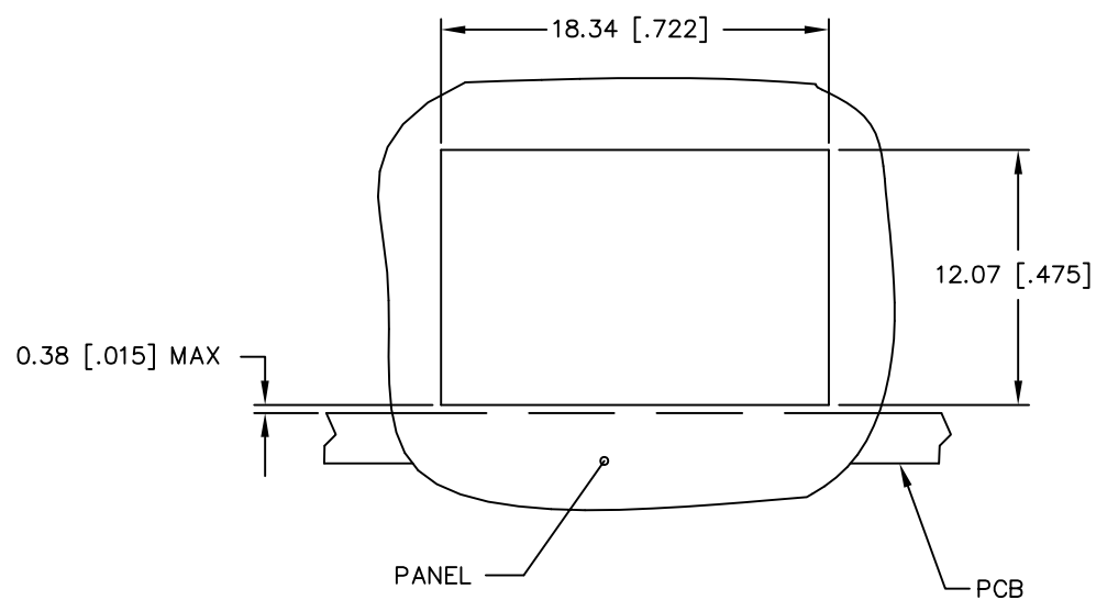
SUGGESTED PANEL CUTOUT
