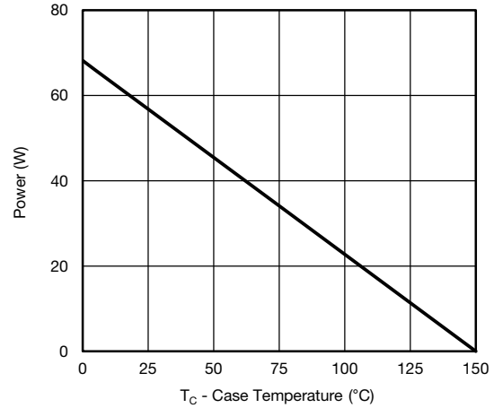
Power, Junction-to-Case
