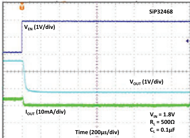
Fig. 33 - Turn-off Time
