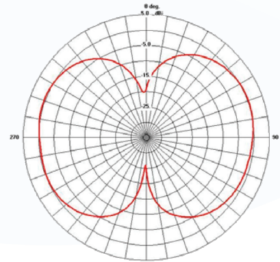
ELEVATION PLANE WCP2400MMCX
