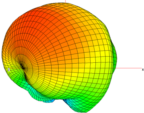
MIMO 1 – 30cmx30cm Ground Plane
