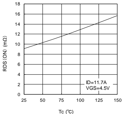
RDS(ON)-Tc characteristics (typical) ID=11.7A, VGS=4.5V
