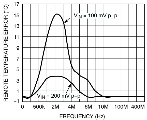
Figure 4. Temperature Error vs. Power Supply Noise Frequency
