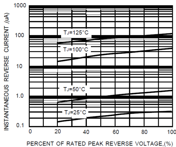
FIG.5-TYPICAL REVERSE CHARACTERISTICS
