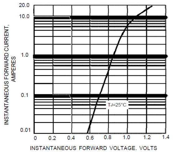
FIG.4-TYPICAL FORWARD CHARACTERISTICS
