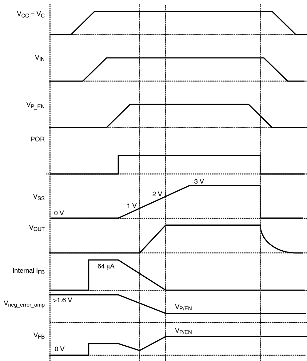
Figure 12. Start-up Sequence
