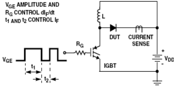
Figure 1. t_{rr} Test Circuit
