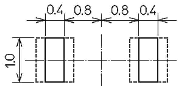
Recommended metal mask hole
