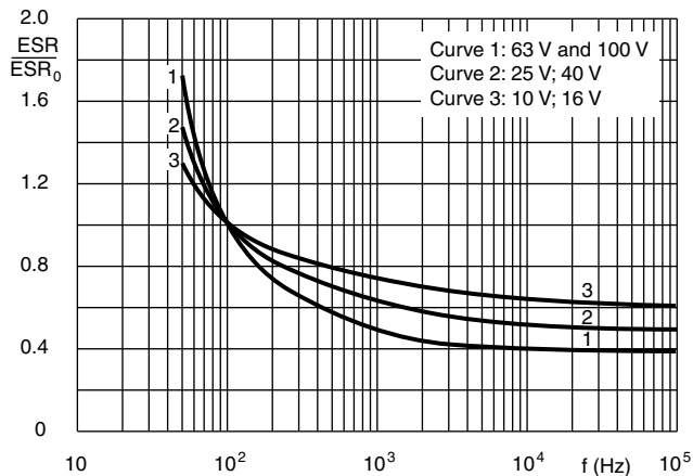
Case \varnothing D \times L = 6.5 \text{ mm} \times 18 \text{ mm} to 10 \text{ mm} \times 25 \text{ mm} ESR 0 = Typical at 20 °C, 100 Hz
