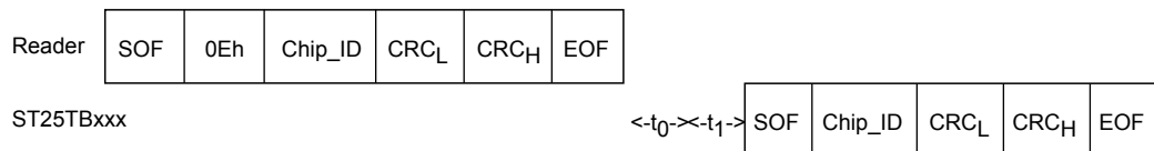
Figure 29. Select frame exchange between reader and ST25TB04K
