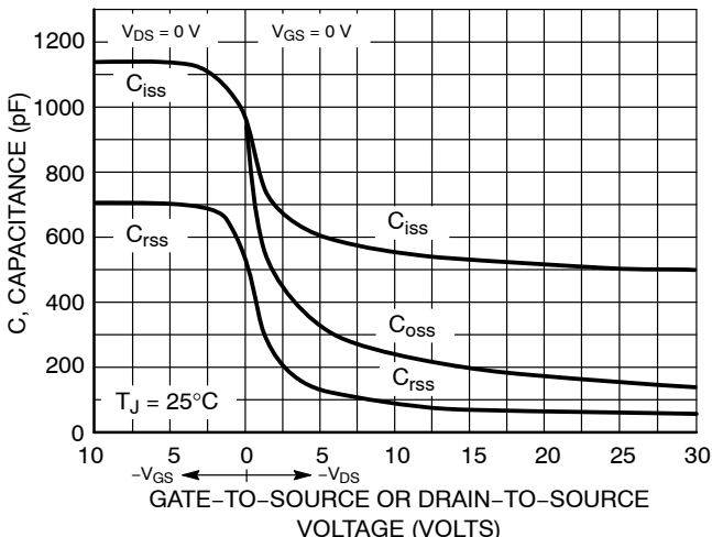
Figure 8. Capacitance Variation
