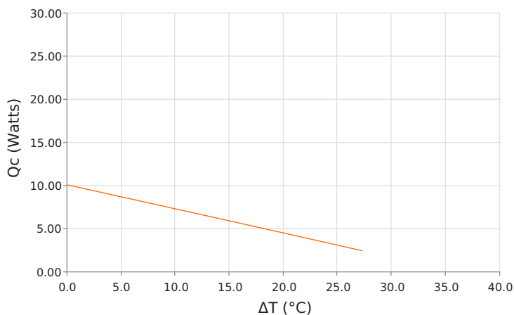
Heat Pumped at Cold Side ( Q_c ) T_{hot} = 85\text{ }^{\circ}\text{C} | Current = 2.1 Amps
