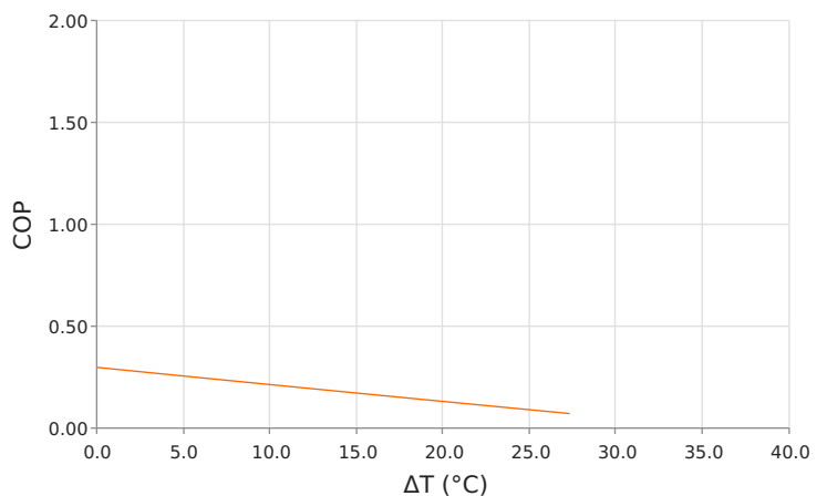
Coefficient of Performance (COP = Q_c/P_{in} ) T_{hot} = 85\text{ }^{\circ}\text{C} | Current = 2.1 Amps
