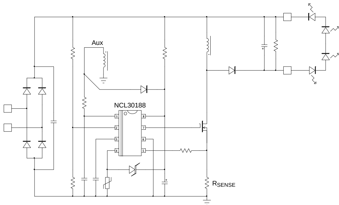
Figure 2. Typical Application Schematic in a Buck-Boost Converter
