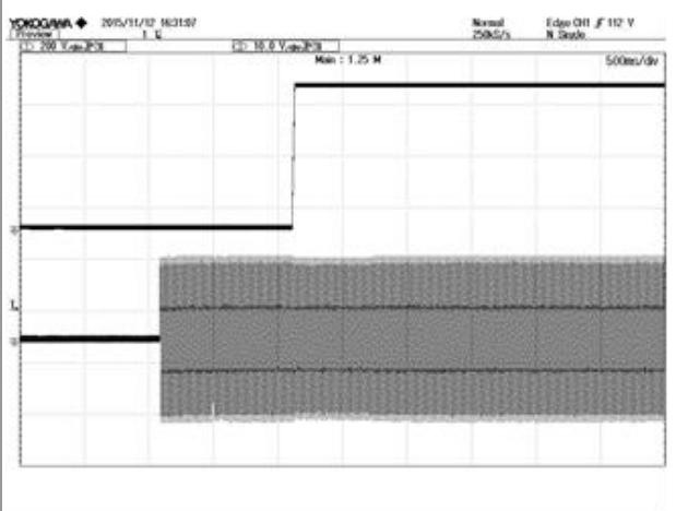
Figure 5: V_{out} start up at 220Vac, 10.5A I_{out} , TOP: VOUT, 10V/div, 500ms/div
