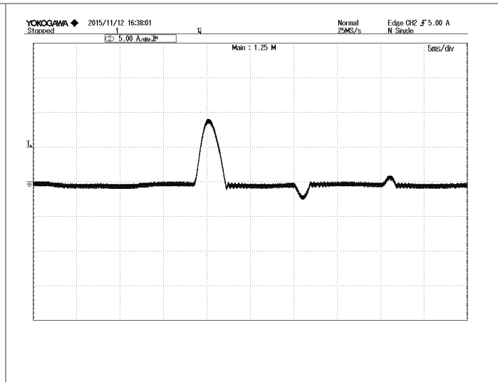
Figure 8: Inrush current @ Vin=220Vac Iin: 5A/div, 5mS/div
