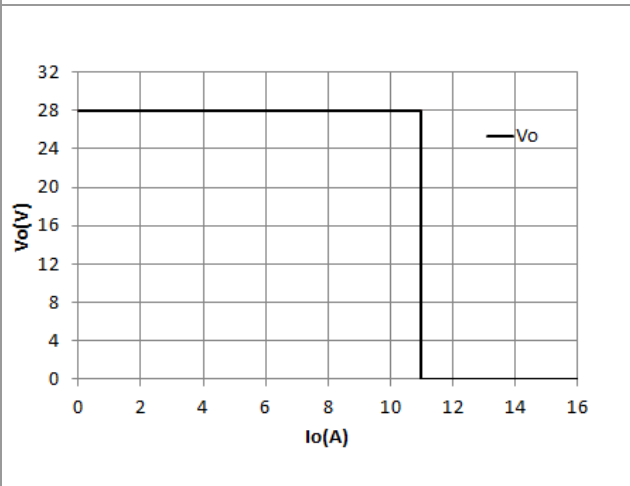
Figure 3: Output voltage vs. Output current @ V_{in}=110/220VAC .
