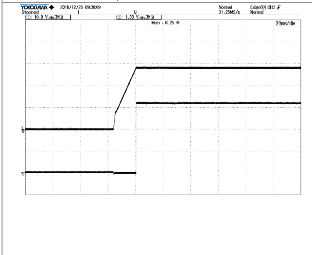
Figure 9: PG voltage vs. Vout @ Vin=220Vac, 0A Iout TOP: Vout, 10V/div, 20mS/div BOTTOM: PG, 1V/div, 20mS/div
