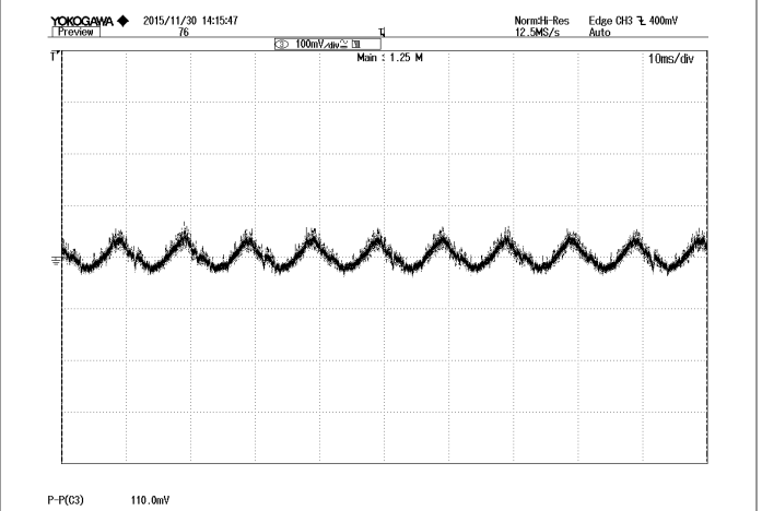
Figure 6: Output ripple & noise at 220Vac, 10.5A I_{out} VOUT: 100mV/div, 10mS/div
