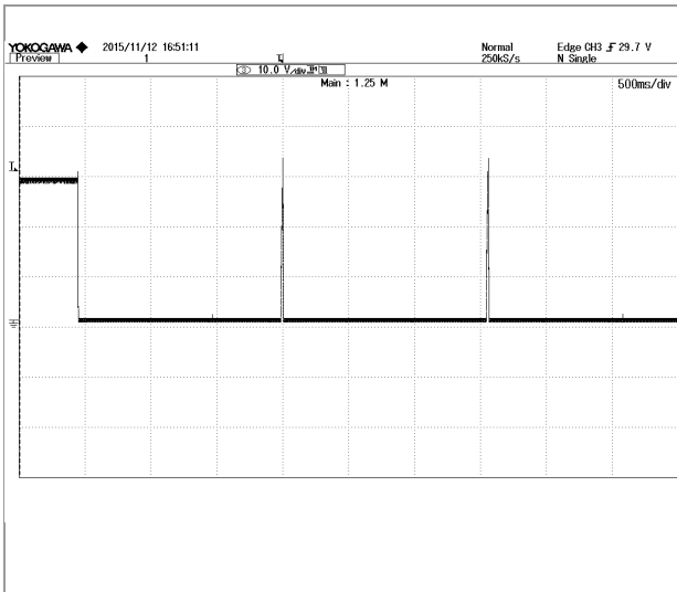
Figure 7: Output over voltage protection at 220Vac, 10.5A Iout. VOUT: 10V/div, 500ms/div
