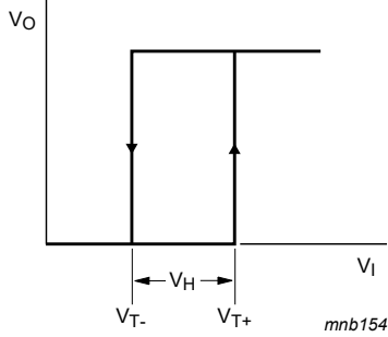
Fig. 14. Transfer characteristic
