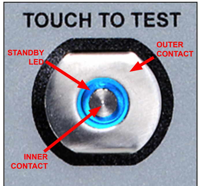
Figure 9. Steady-State Test Switch features and components
