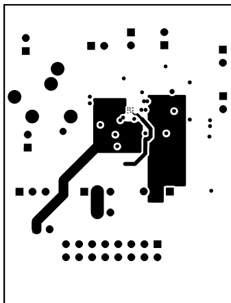
Figure 47. Internal Layer 2
