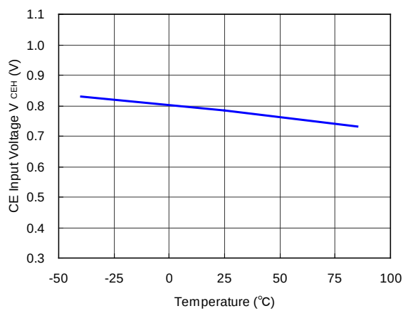
CE“H” Input Voltage ( V_{IN} = 5.5 \text{ V} )
