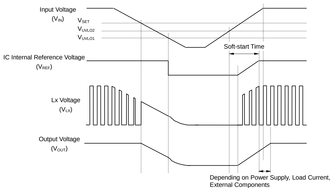
Timing Chart
