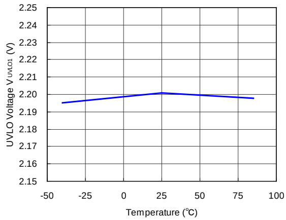
UVLO Detector Threshold
