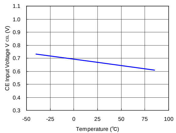
CE“L” Input Voltage ( V_{IN} = 2.5 \text{ V} )
