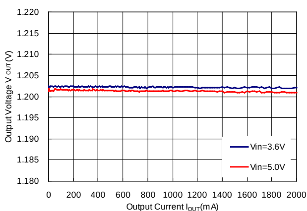
RP506Kxx1D/E/F V_{OUT} = 1.2\text{ V} MODE = "H" Forced PWM Control
