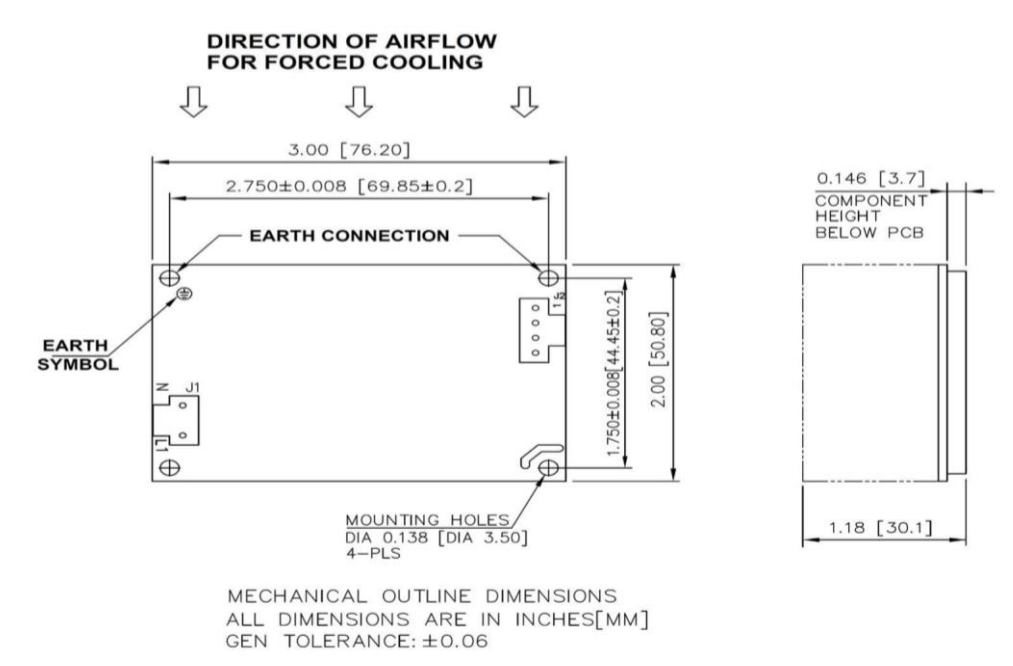
Figure 3. Mechanical Drawing - Molex Header (Option 2)
