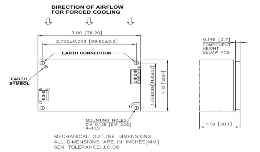
Figure 2. Mechanical Drawing - Screw Terminal (Option 1)
