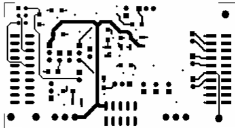
Figure 2-6. Bottom Silkscreen
