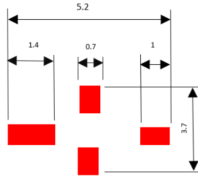
PCB Footprint
