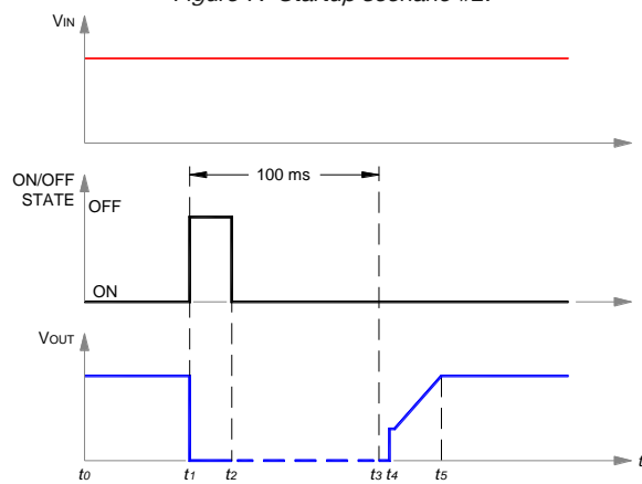
Figure 8. Startup scenario #3.
