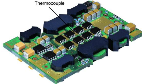
Figure 27. Location of the thermocouple for thermal testing.
