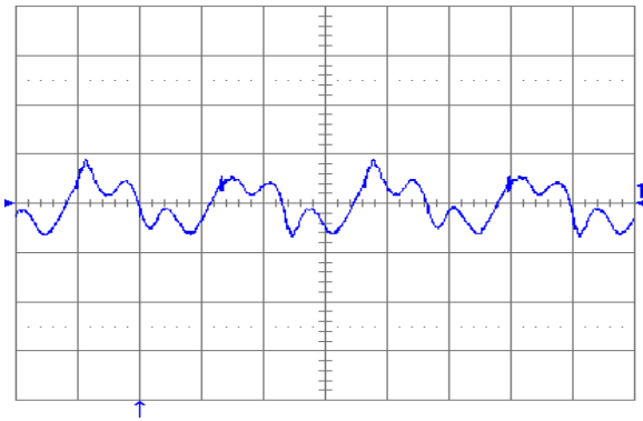
Figure 21. Output voltage ripple (20 mV/div.) at full rated load current into a resistive load with C_o = 10 \mu F tantalum + 1 \mu F ceramic and V_{in} = 48 V. Time scale: 1 \mu s/div.
