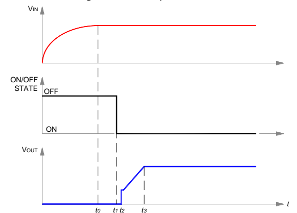
Figure 7. Startup scenario #2.
