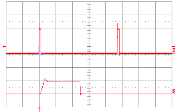
Figure 26. Load current (top trace, 20 A/div, 20 ms/div) into a 10 mΩ short circuit during restart, at V_{in} = 48 V. Bottom trace (40 A/div, 1 ms/div) is an expansion of the on-time portion of the top trace.
