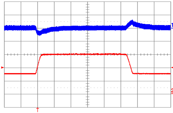
Figure 19. Output voltage response to load current step-change (7.5 A – 15 A – 7.5 A) at V_{in} = 48 V. Top trace: output voltage (100 mV/div). Bottom trace: load current (5 A/div). Current slew rate: 0.1 A/ \mu s. C_o = 1 \mu F ceramic. Time scale: 0.2 ms/div..
