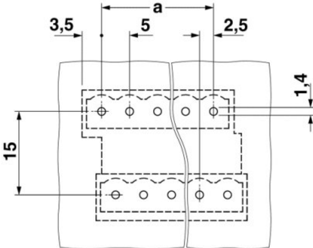
Drilling diagram
